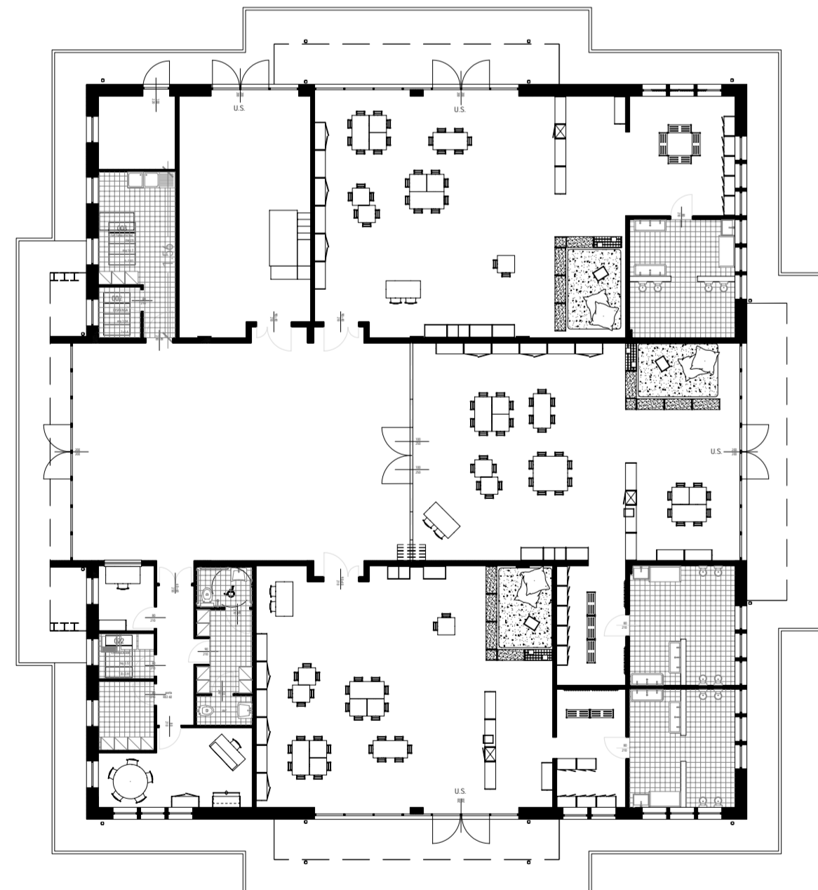
layout arredi 1/200
